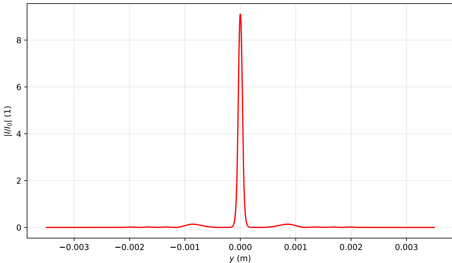
Intensity profile I(x=0, y, z=0.637)/I_0 , P_{in}=7.0P_{cr} , artificial time
